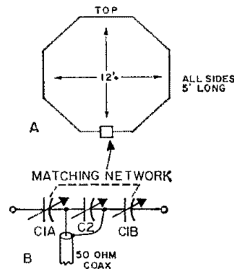
Fig. 1—A—Drawing of the octagonal loop; B—The matching network. In matching, a 50-ohm s.w.r. bridge is inserted in the coaxial line and the network adjusted to a 1-to-1 match.
