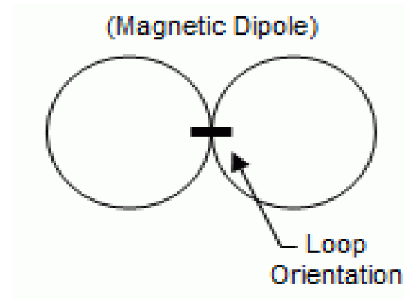
Radiation pattern
