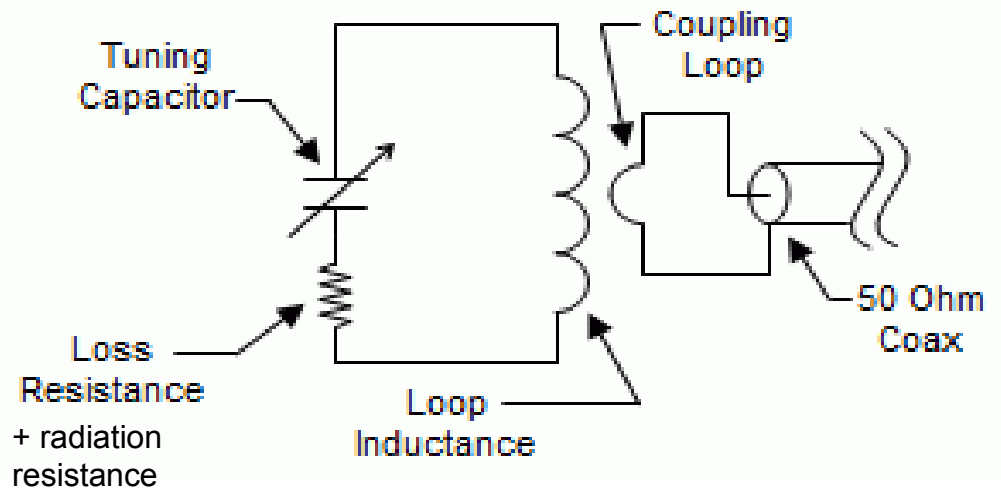
Equivalent circuit
